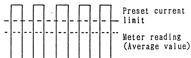
Figure 2-7 Equivalent Circuit of Pulse Waveform
